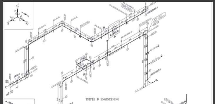
DESIGN ENGINEERING OF PIPING
