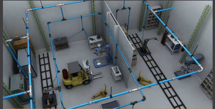
PNEUMATIC PIPING
